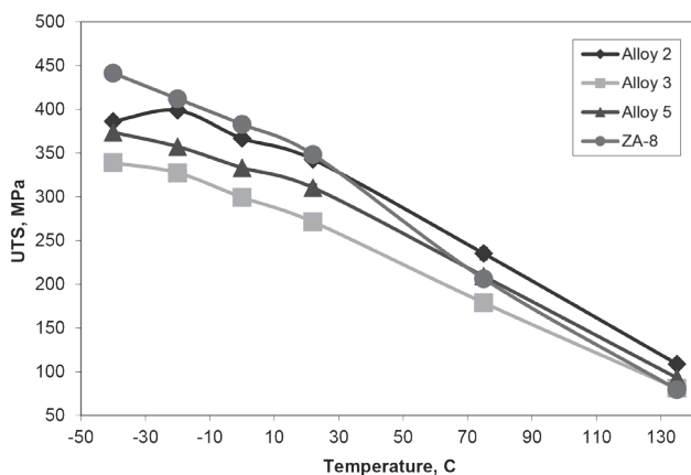
Zinc Tensil Strength at Temperature
